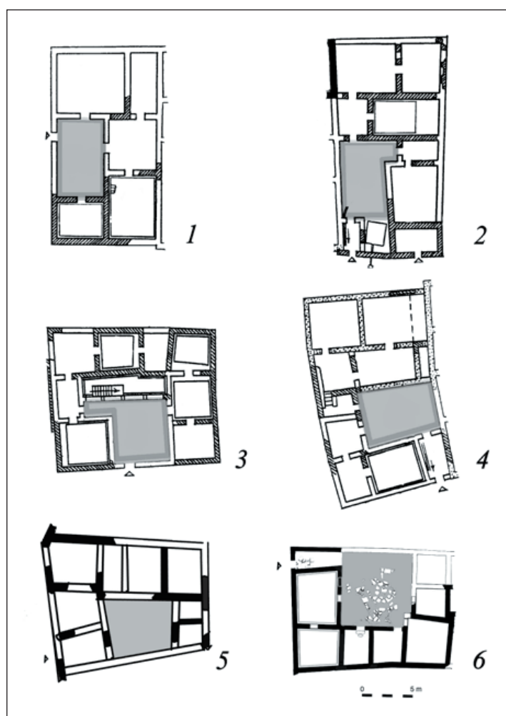
2 • Houses with Π-shaped arrangement of rooms: 1: House A-4; 2: House A-3; 3: House E-1; 4: House E-2; 5: House E-6; 6: Sector NGS, House II-3.
