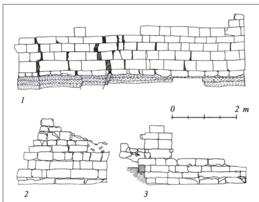
2 • Single-row of orthogonal plates and blocks. 1: Wall 318; 2: Wall 71; 3: Wall 72.
